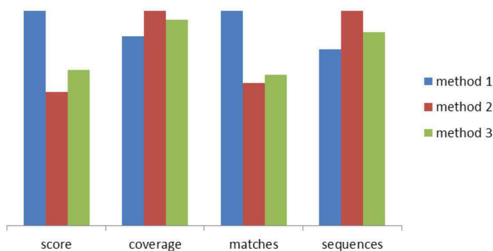
Figure 1: Comparison of three sample preparation methods on a fresh paint sample with rabbit skin glue, showing significant differences in protein scores, protein coverage, number of matched spectra and number of non-identical peptide sequences for collagen type 1 alpha 1.
